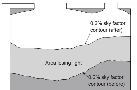
Figure E1: Plan of room showing movement of the 0.2% sky factor contour following erection of an obstruction
