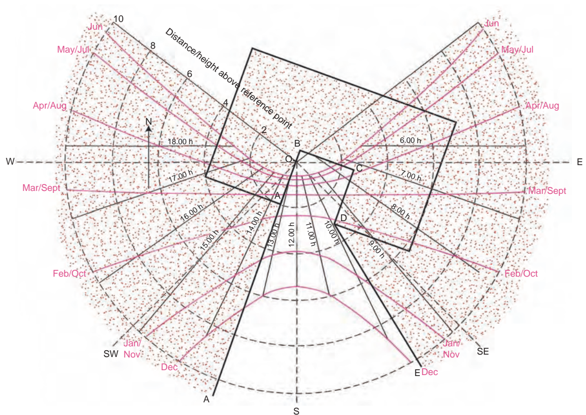
Figure A17: Direction finder plot of housing layout (Figures A9 and A10) laid over sunpath indicator
