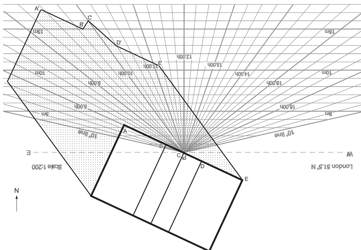
Figure G5: Use of the sun-on-ground indicator to plot the shadow of the example building in Figure G4 on 21 March
