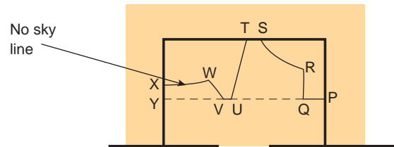
Figure D6: For a general horizontal obstruction, part of the no sky line runs parallel to the obstruction. The rest runs along the projected lines from the ends of the obstruction through the corners of the window.
