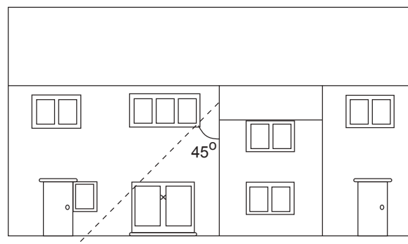
Figure 16: To assess the impact of the new extension, the 45° approach may be used for window A but not for windows B and C which directly face it
