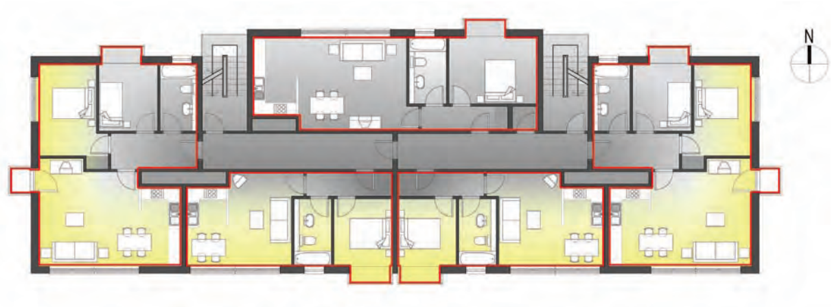
Figure 26: Careful layout design means that four out of the five flats shown have a south-facing living room
