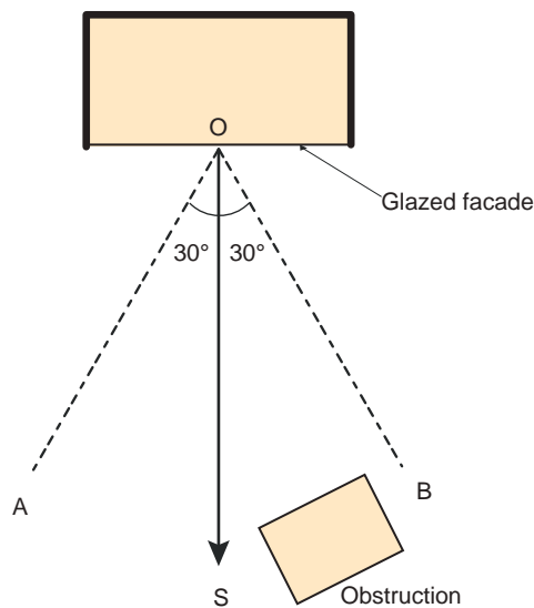
Figure 35: For passive solar gains in winter the sector AOB 30^\circ either side of due south is important. To guarantee winter sun from this sector, obstructions within it should not subtend more than the critical angle h when measured in section. Table 1 gives values for h .
