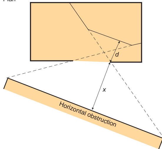
Figure D6: For a general horizontal obstruction, part of the no sky line runs parallel to the obstruction. The rest runs along the projected lines from the ends of the obstruction through the corners of the window.
