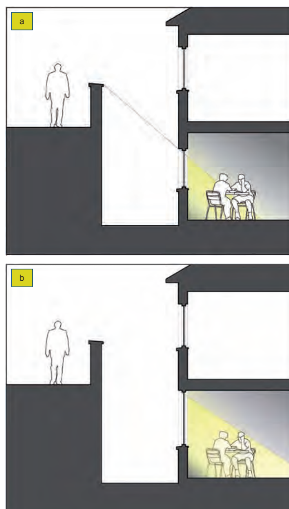
Figure 4: Daylight penetration in a basement (a) is improved by a raised window head (b)
