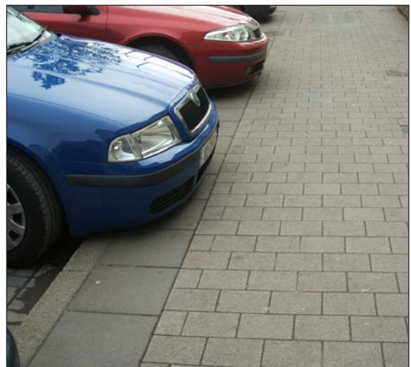
Figure 4.36: An example where a narrow verge is provided to ensure that vehicle overhangs do not intrude on the footway.
