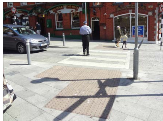
Figure 4.24: Example from Drogheda, Co. Louth, of red tactile paving at a zebra crossing which has been toned down to balance the degree of contrast with higher specification materials.
