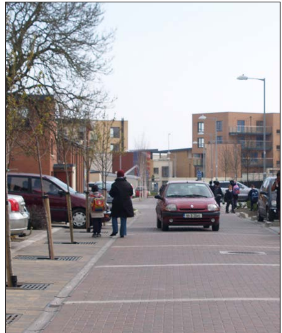
Figure 4.51: Examples from Adamstown, Co. Dublin, where a verge is provided as refuge that pedestrians can hop on and hop off as cars slowly pass.
