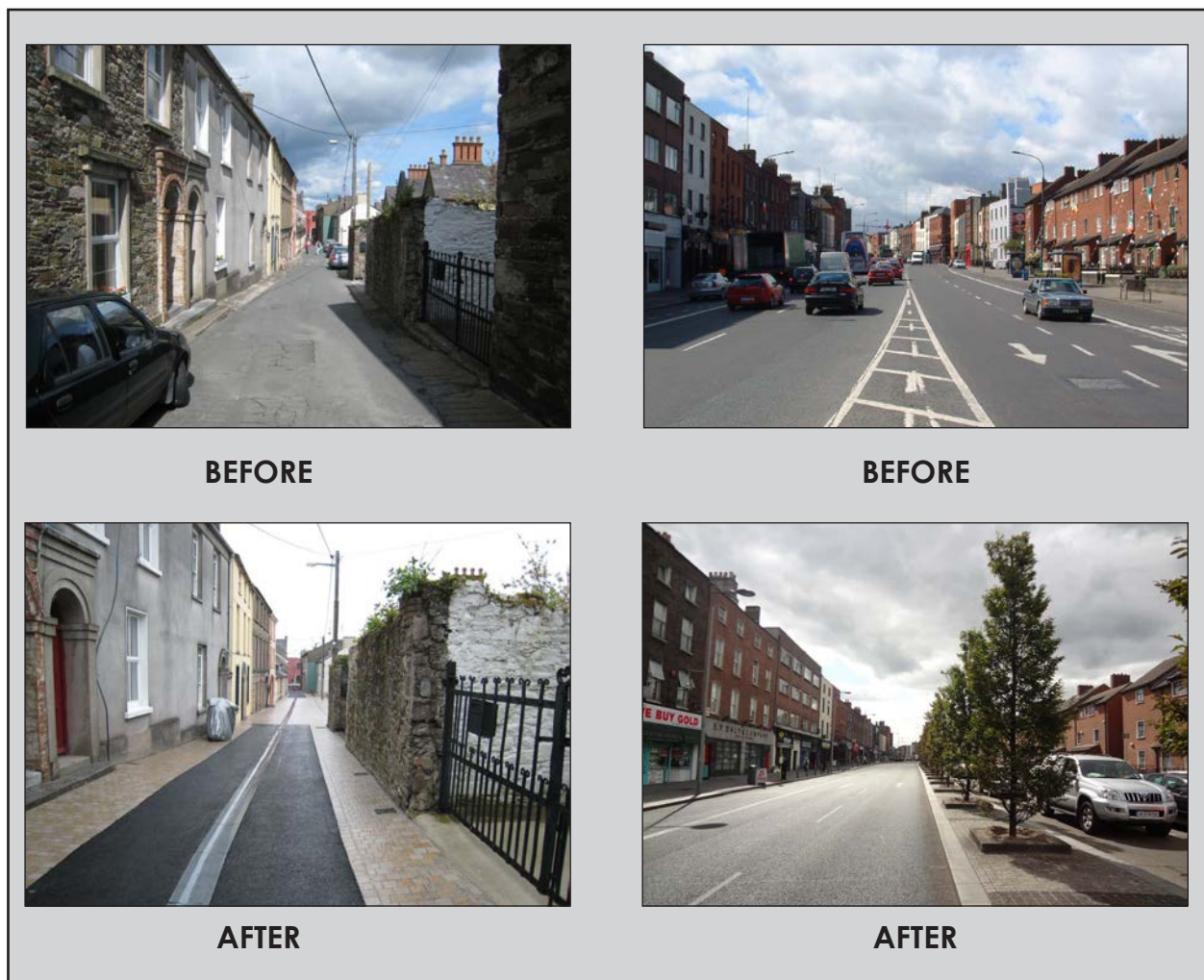
Figure 4.6: Examples from Youghal, Co. Cork (left), and Dorset Street, Dublin City (right), of retrofitted design responses that are appropriate according to Context and Function. The narrow, enclosed and lightly trafficked nature of the street within Youghal is highly suited to a shared carriageway. The heavily trafficked nature of Dorset Street makes it highly suited to a Boulevard type configuration.
